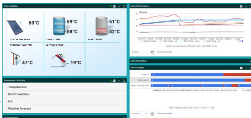
With Cm WiFi-box (additional equipment) controll solar system through mobile phone / tablet / PC.
